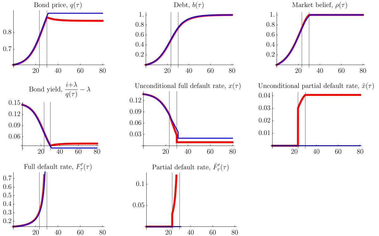
Figure 3: Equilibrium path starting from \rho_0 = 0 and b_0 = 0 . H is as in equation (17). The rest of the parameters are y = 1 , \epsilon = 0.1 , \delta = 0.02 , i = 0.01 , \lambda = 0.2 , b^* = 0.5 , and \theta = 0.03 . Values for \tau^* and T are represented by vertical lines. The partial default model is displayed using red lines, and the original model is displayed using blue lines.
